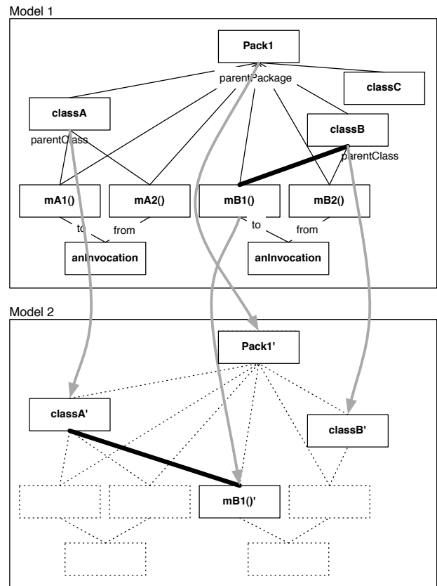
Figure 6. LookUp/Pointer Approach
